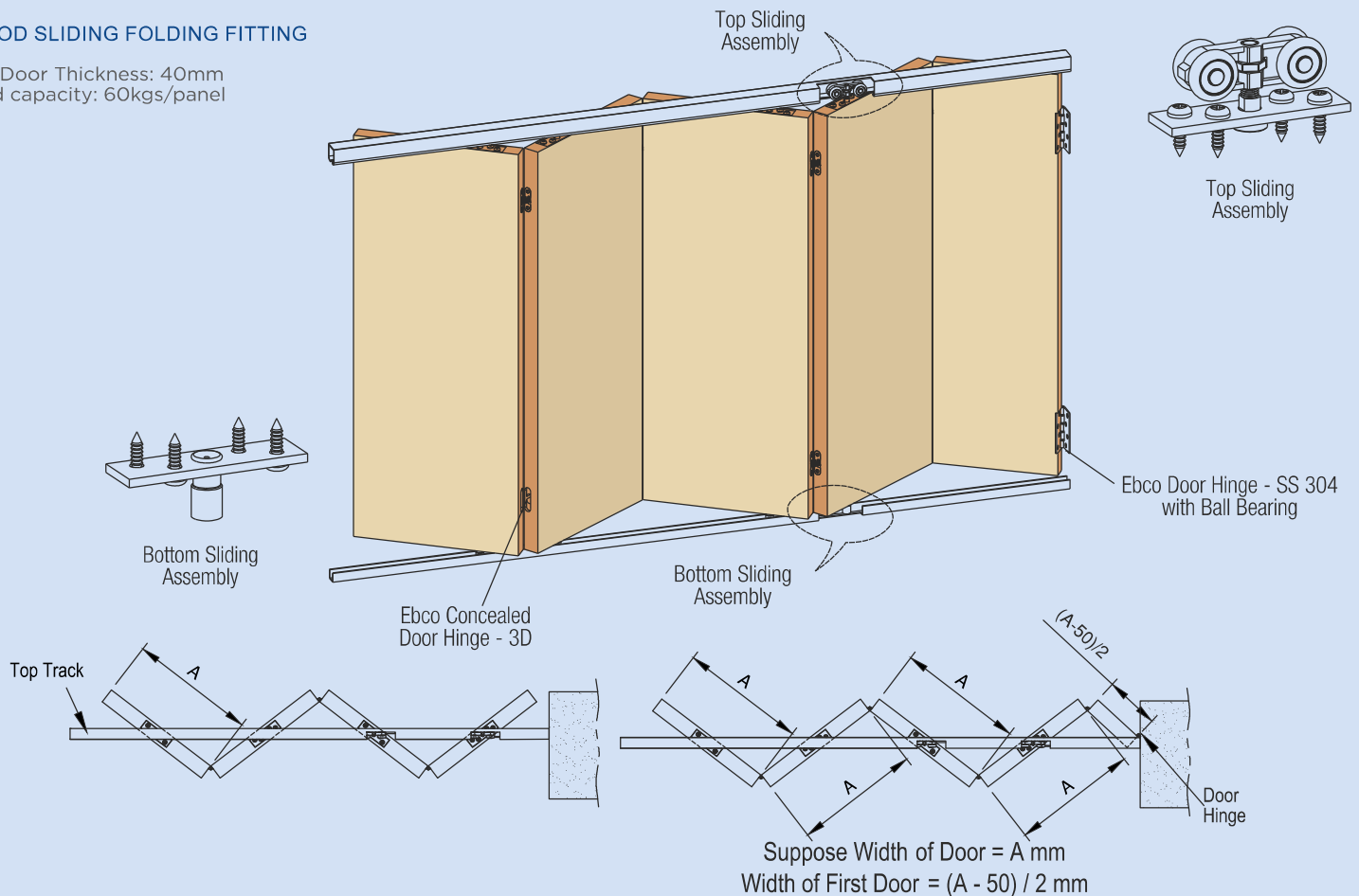
Wooden Door
