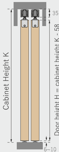
Wooden Door
