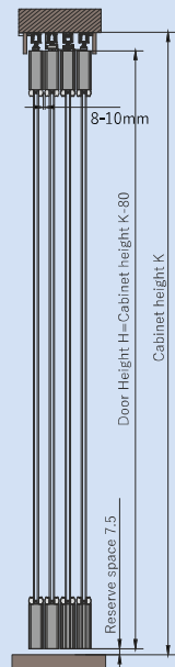
Wooden Door
