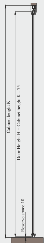
Al. Frame Door
