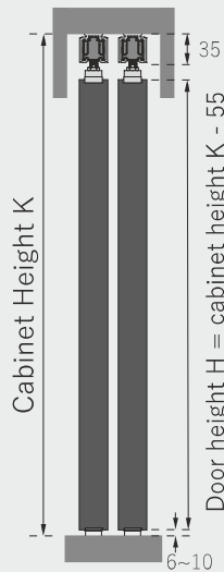
Al. Frame Door
